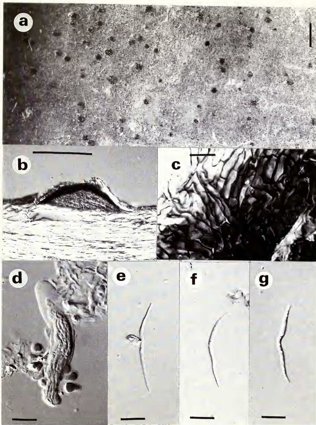
Fig. 14 Leptorhaphis maggiana (Massal.) Körber (BM-lectotype) (a) Surface view; scale = 500 \mu\text{m} ; (b) Vertical section of ascoma; scale = 100 \mu\text{m} ; (c) Detail of involucrellum (surface view): textura epidermoidea-intricata; (d) Ascus and ascospores; (e), (f), (g) Ascospores; scale = 10 \mu\text{m} .
